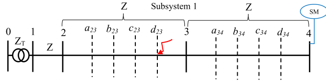
Fig. 4. Subsystem 1 with fictitious buses.
