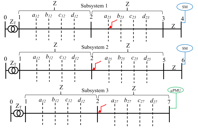
Fig. 5. Subsystems 1, 2, and 3 with fictitious buses at different sections.
